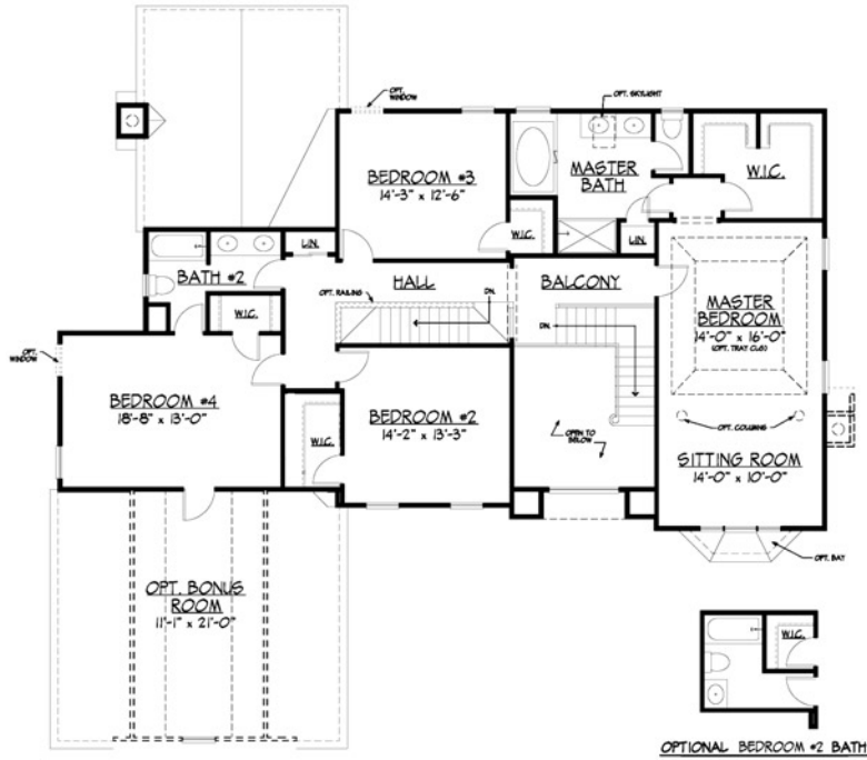
Second Floor Plan with Optional Bonus Room
